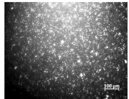
Figure 4. Fluorescence microscopy (zoom \times 200 ) images of bitumen after ageing (RTFOT + PAV)
