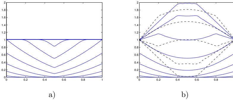
Figure 1. Behavior with respect to time (left) of the function E = E_z in (3.1) with V obtained from (3.5). This is compared (right) with the solution of the wave equation (1.5) corresponding to the same boundary data. Inconsistent oscillations are produced in the second case, where the initial transient (solid lines) is followed by a periodic regime (dashed lines). The principal modes ( \sin \pi z and \sin 3\pi z ) are clearly visible.
