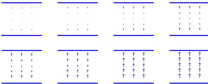
Figure 2. Displacement of the electric field \mathbf{E} during the charge of a capacitor. The divergence of \mathbf{E} remains different from zero, until the process is terminated.
