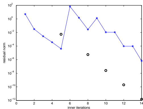
Figure 2. Convergence history; quadratic eigenproblems by Arnoldi algorithm.
